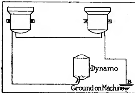
Fig. 3—Wiring diagram for electric headlights on Ford car
